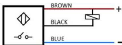
NPN NORMALLY OPEN
