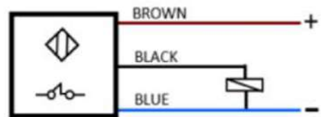
PNP NORMALLY CLOSE
