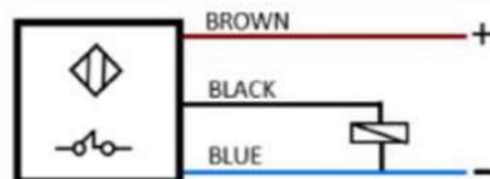
PNP NORMALLY CLOSE
