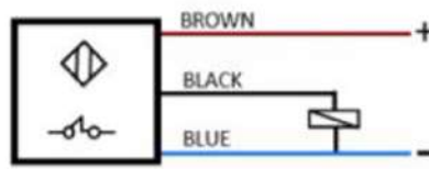
PNP NORMALLY CLOSE
