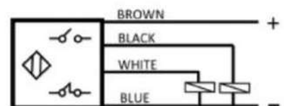
PNP 1NO+1NC
